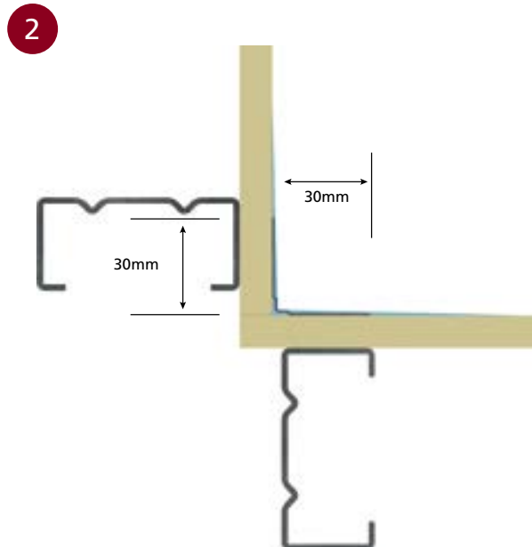
■ INTERNAL CORNER BEAD DETAIL
