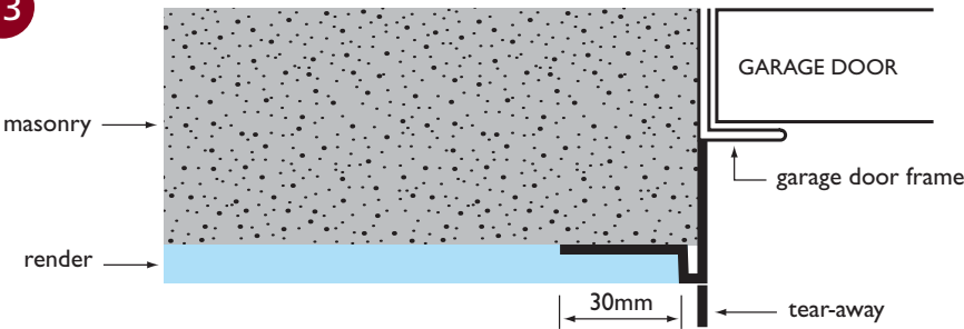
■ RTLB102530 DETAIL
