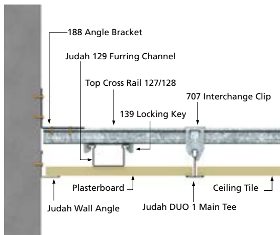
■ ALTERNATIVE PERIMETER DETAIL
