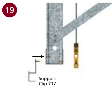
■ SUPPORT CLIPS
