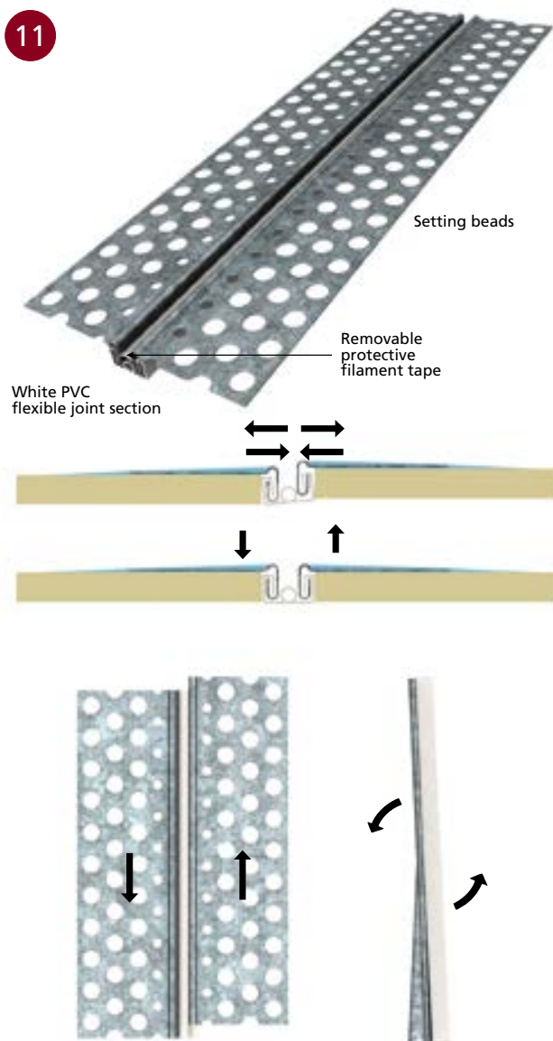
■ P35 CONTROL JOINT
