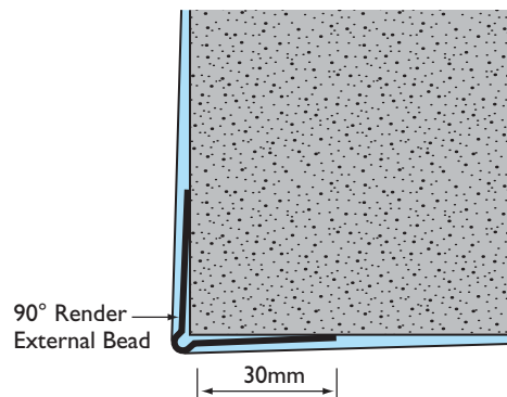
■ RE9025 DETAIL
