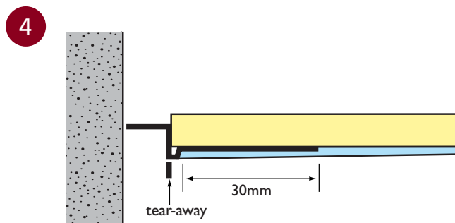
■ PTSH1030 DETAIL
