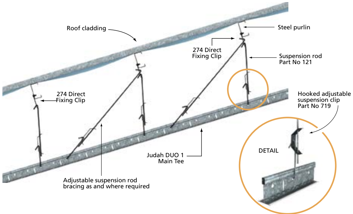
■ SUGGESTED RAKING CEILING DETAIL (maximum pitch: 45°)
