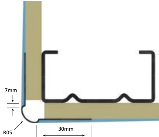
■ R05 INSTALLATION DETAIL
