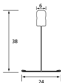
Judah DUO 1 24mm MAIN TEE
