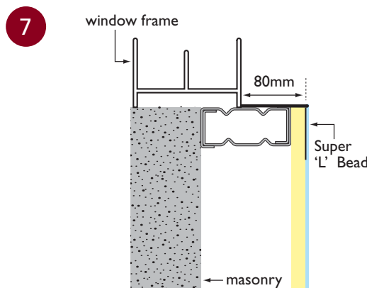
■ PSLB8030 DETAIL
