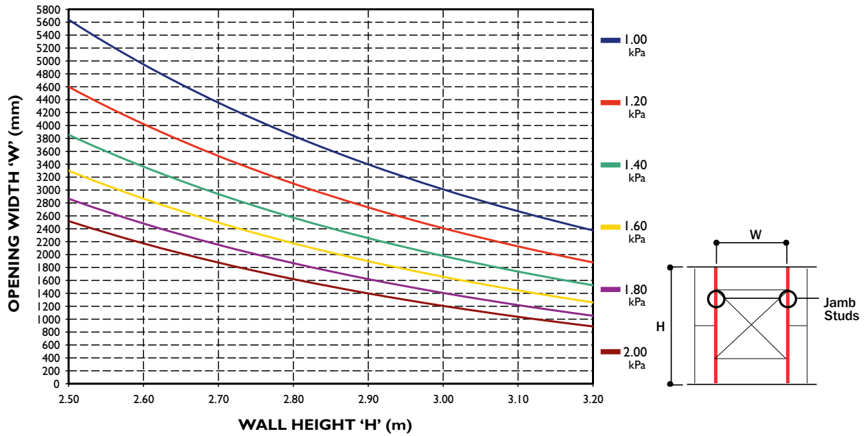
CHART J1: DESIGN REGION A — H/240
