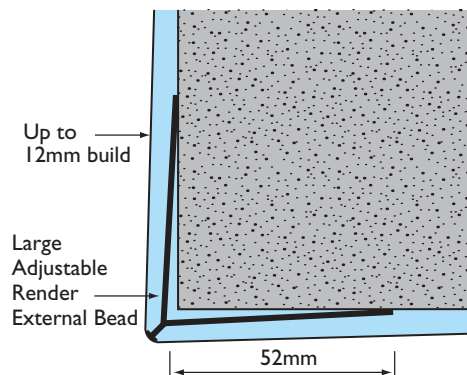
■ RELA30 DETAIL
