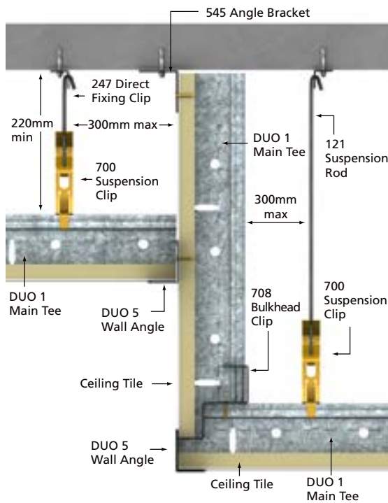
■ SQUARELINE BULKHEAD DETAIL (Vertical Exposed Grid)
