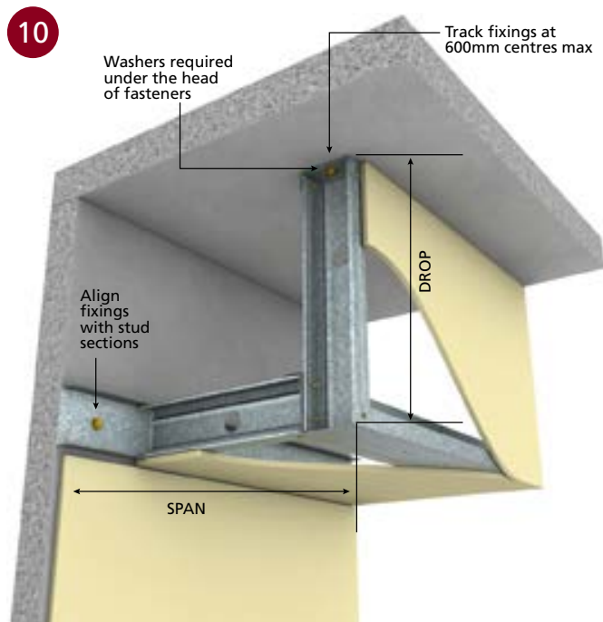
■ BOX-TYPE BULKHEAD
