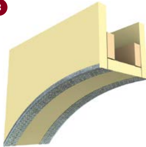
■ ARCH BEAD: TYPICAL APPLICATION
