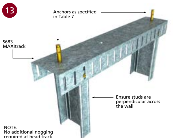
■ TYPICAL MAXITRACK CONNECTION DETAILS
