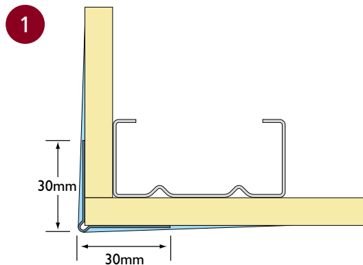
■ EXTERNAL CORNER BEAD DETAIL
