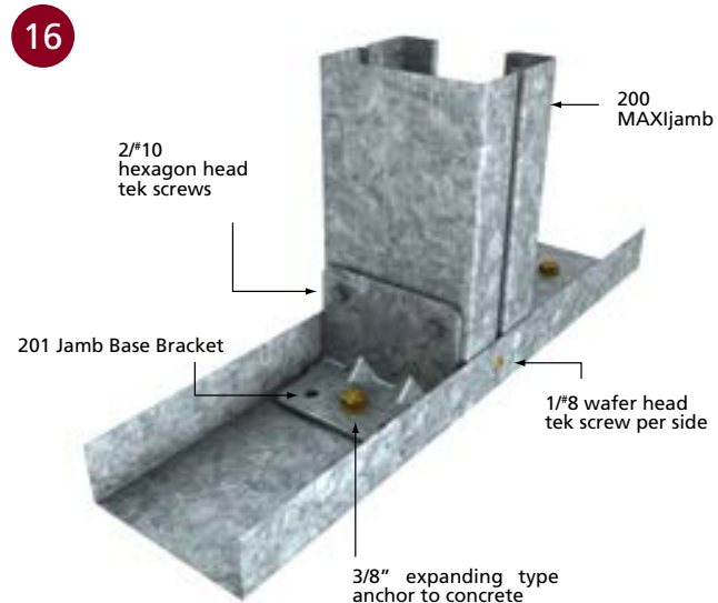
■ TYPICAL MAXIJAMB BASE FIXING DETAILS
