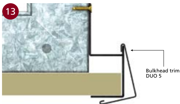
■ BULKHEAD TRIM
