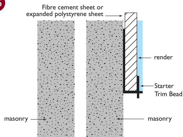
■ RENDER STARTER BEAD DETAIL
