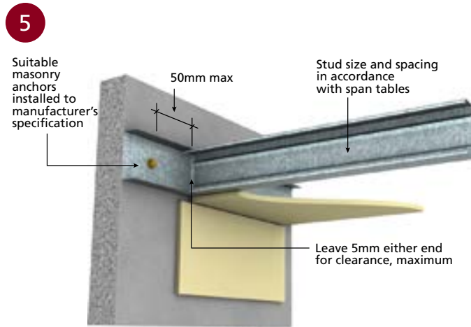
■ FRICTION JOINT
