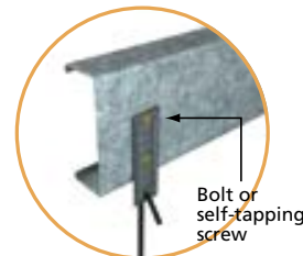
Suspension rod bracket Part No 547
