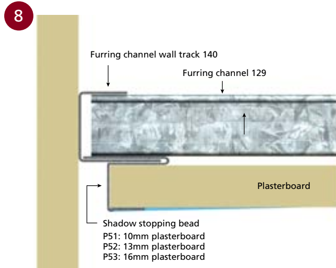
■ SHADOW SET DETAIL
