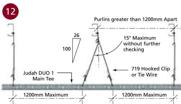
■ SPANS GREATER THAN 1200MM
