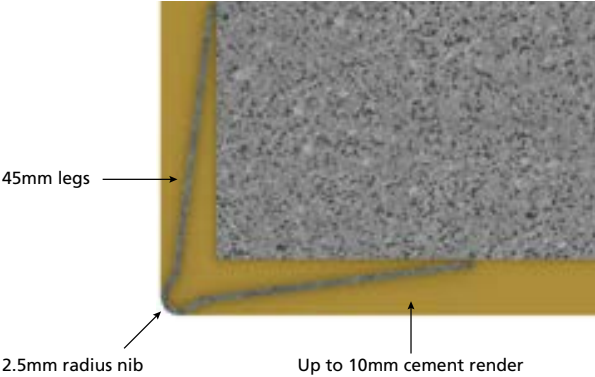
■ SR02 CORNER BEAD DETAIL
