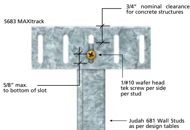
■ TYPICAL MAXITRACK FIXING DETAIL
