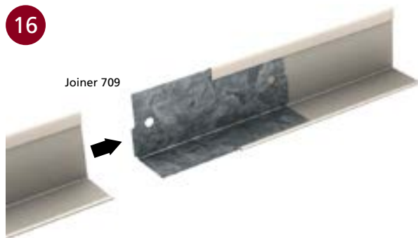
■ BULKHEAD JOINER DETAILS
