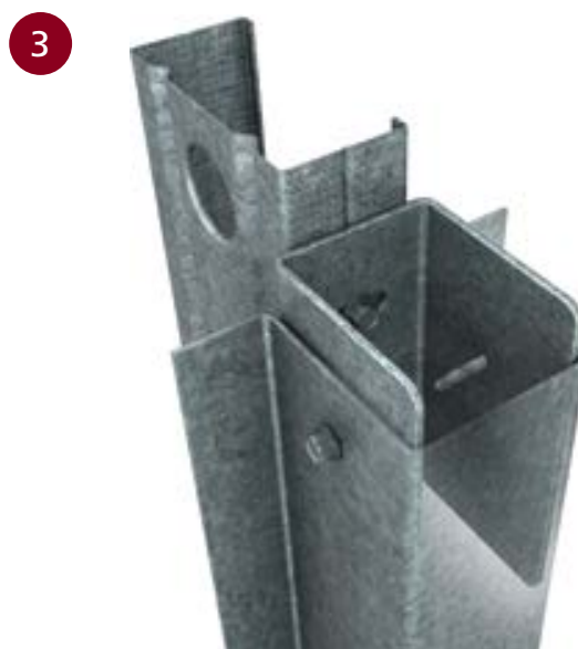
■ VERTICAL FIXING METHOD USING CLEAT
