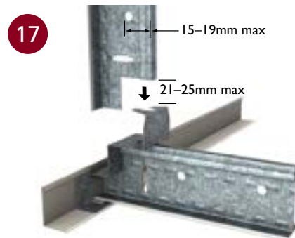
■ VERTICAL MEMBERS
