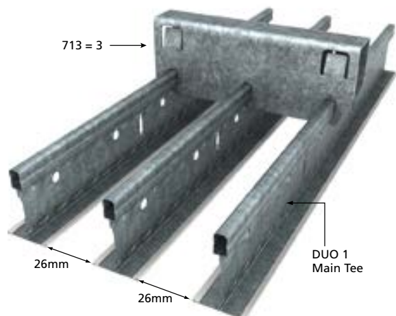
■ AIR DIFFUSER DETAIL
