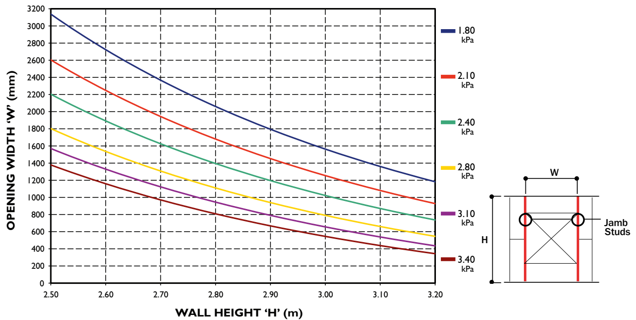
CHART J4: DESIGN REGION B — H/360
