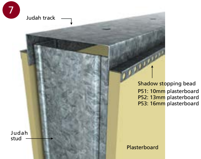
■ SHADOW STOPPING BEAD: TYPICAL APPLICATION
