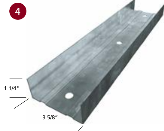
■ 680 WALL TRACK
