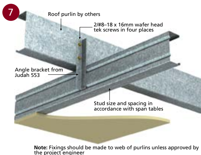
■ SUSPENSION JOINT TYPE 2
