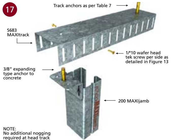
■ EXPLODED VIEW OF MAXIJAMB HEAD CONNECTION
