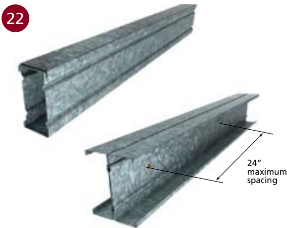
BOXED AND BACK-TO-BACK STUD SECTIONS
