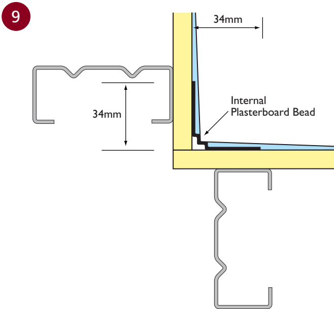
■ INTERNAL PLASTERBOARD BEAD DETAIL
