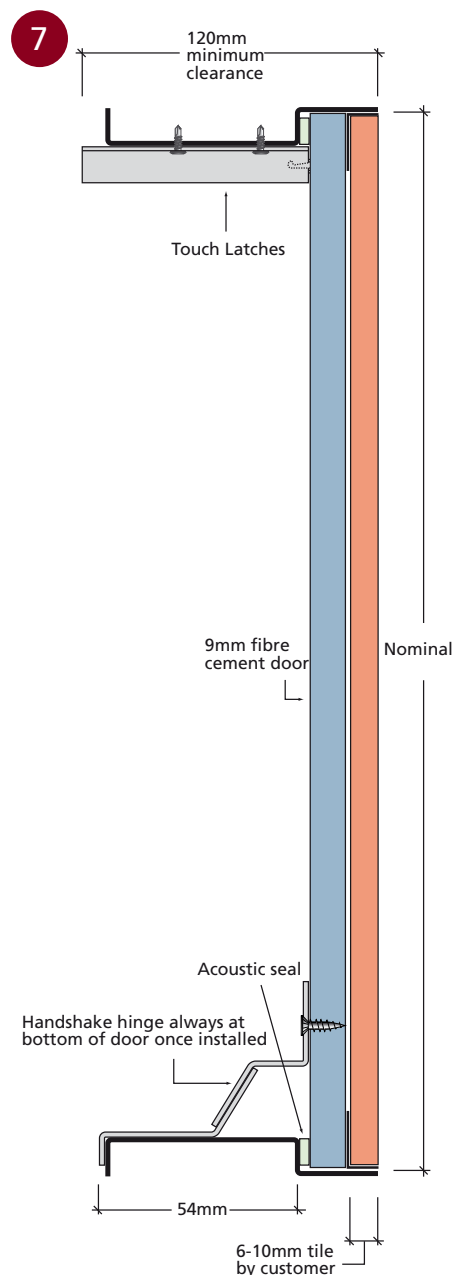
■ INSTALLATION DETAIL
