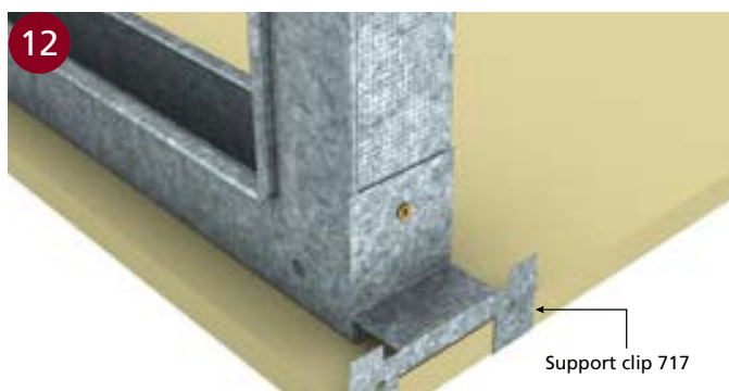
■ SUPPORT CLIPS
