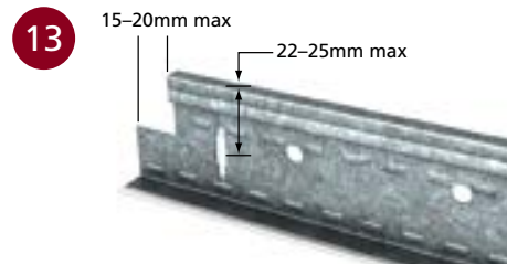
■ HORIZONTAL FRAMING MEMBERS
