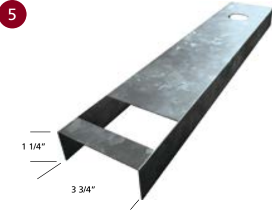
■ 506 NOGGING TRACK
