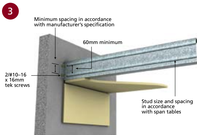
MECHANICAL JOINT TYPE 2
