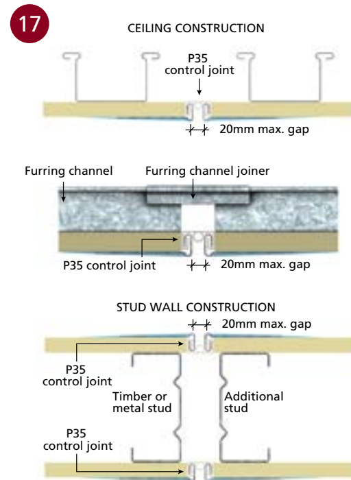
■ P35 INSTALLATION
