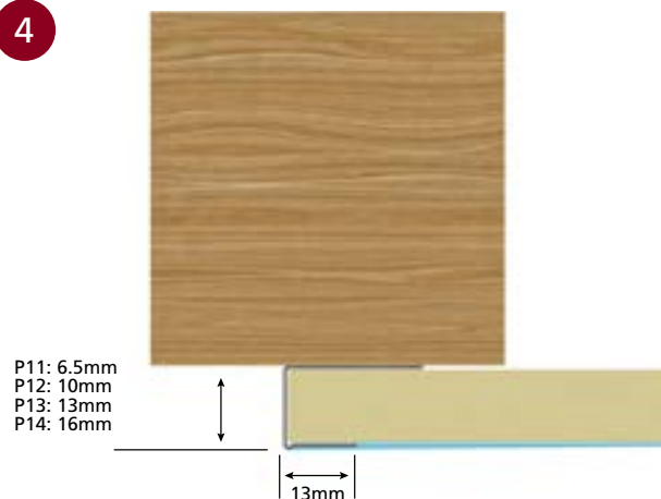
■ STOPPING BEAD DETAIL
