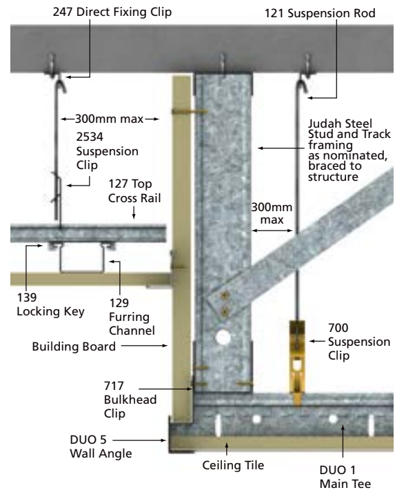
■ SQUARELINE BULKHEAD DETAIL (Vertical KEY-LOCK®/Steel Stud System)
