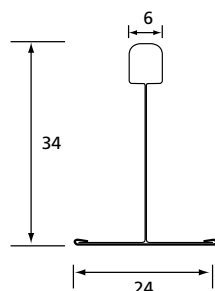
Judah DUO 2/DUO H 24mm CROSS TEE
