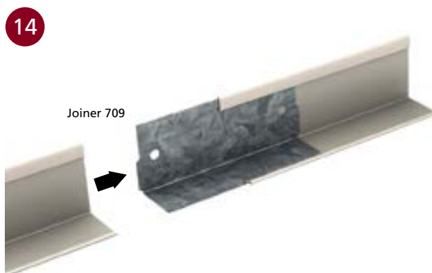
■ BULKHEAD DETAILS
