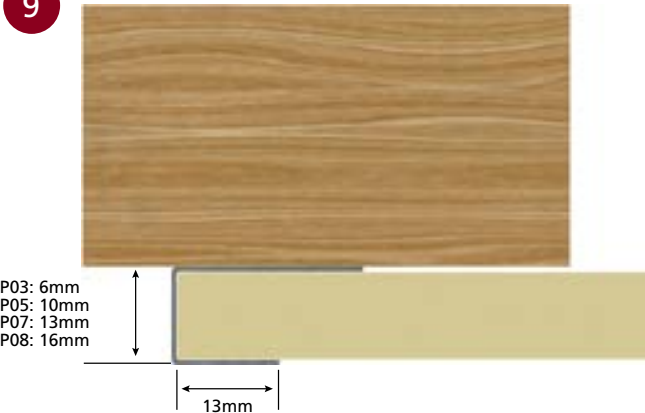
CASING BEAD DETAIL
