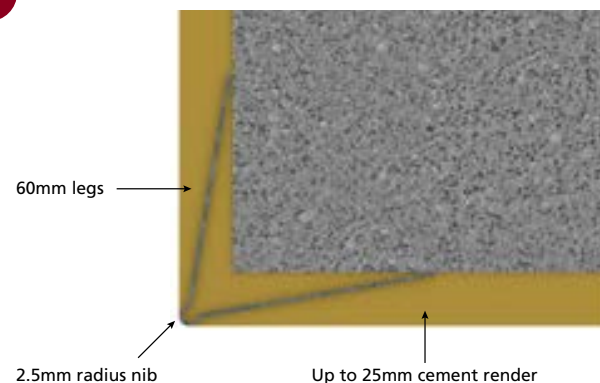
■ R02 CORNER BEAD DETAIL
