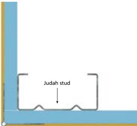
EP32 DETAIL
