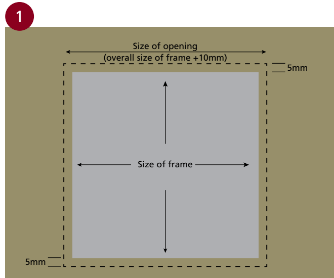
■ CUTTING HOLE IN LINING BOARD
