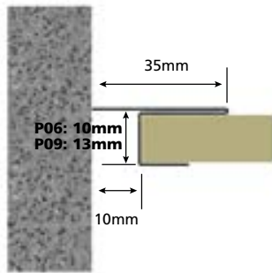
SHADOWLINE CASING BEAD DETAIL
