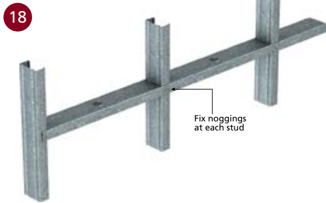
18 NOGGING DETAILS
