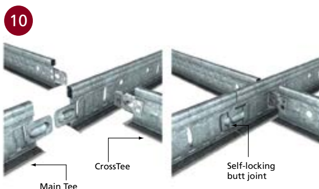
■ TEE JOINTING DETAILS
