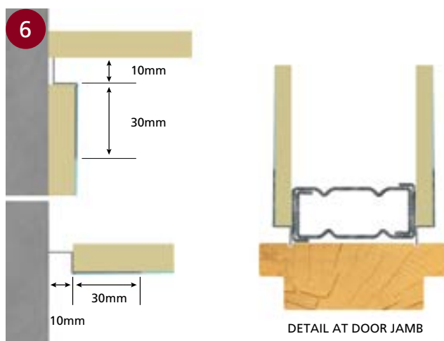
■ SHADOWLINE STOPPING ANGLE DETAIL
