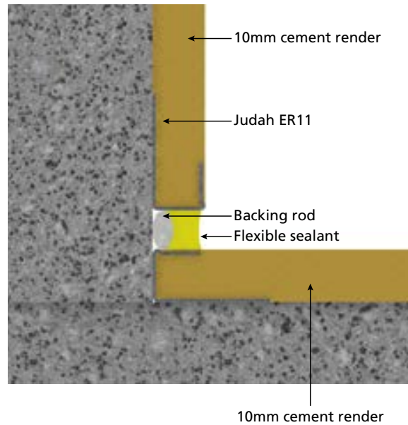
■ CORNER DETAIL
