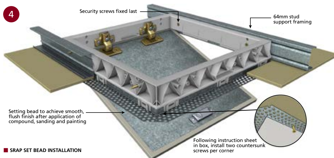
■ SRAP FLANGED INSTALLATION
