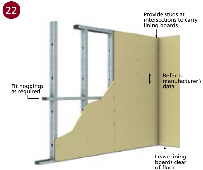
■ VERTICAL APPLICATION
