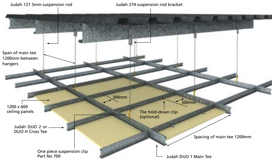
■ TWO-WAY EXPOSED CEILING SYSTEM DETAIL
