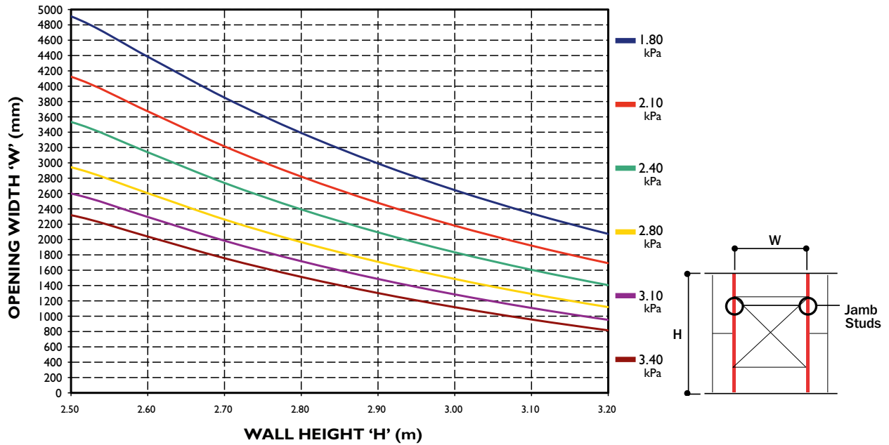
CHART J3: DESIGN REGION B — H/240
