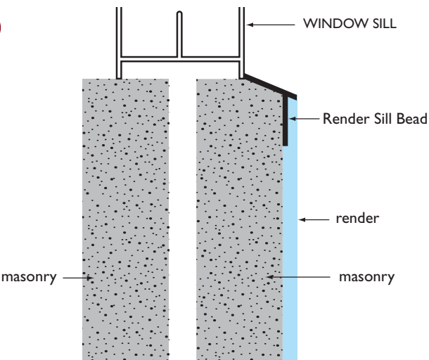
■ WINDOW SILL BEAD DETAIL
