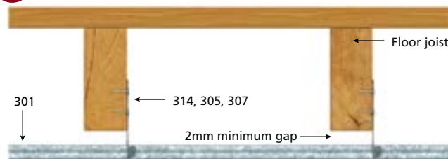
TRAFFICABLE FLOOR INSTALLATION DETAIL
