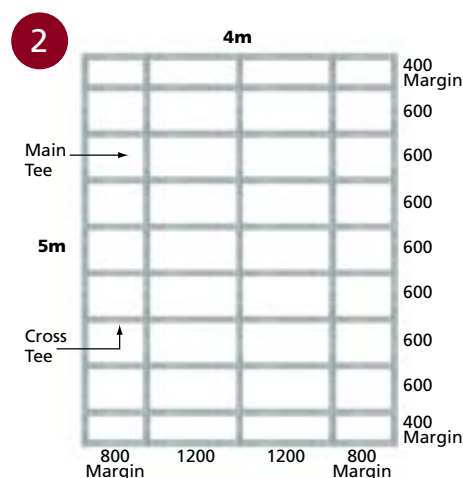
■ WORKING OUT EVEN MARGINS (as per example shown)
