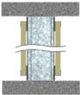
PARTITION FLOOR/HEAD TRACK DETAIL
