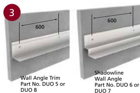
■ PERIMETER WALL ANGLE TRIM
