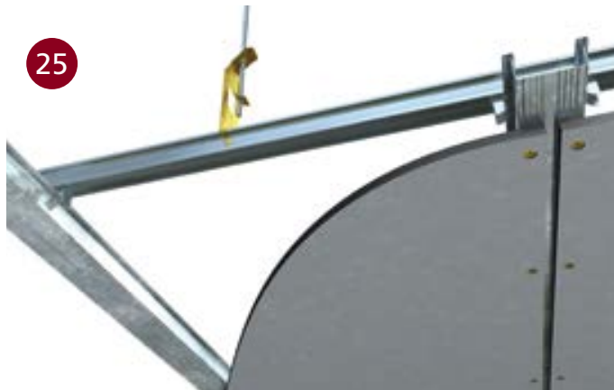
■ 155 USED IN INTERNAL CEILING
