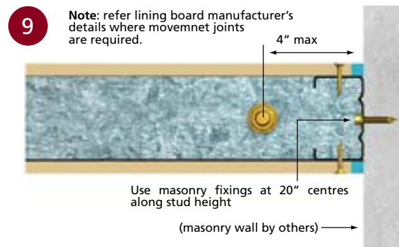
■ INTERSECTION - MASONRY
