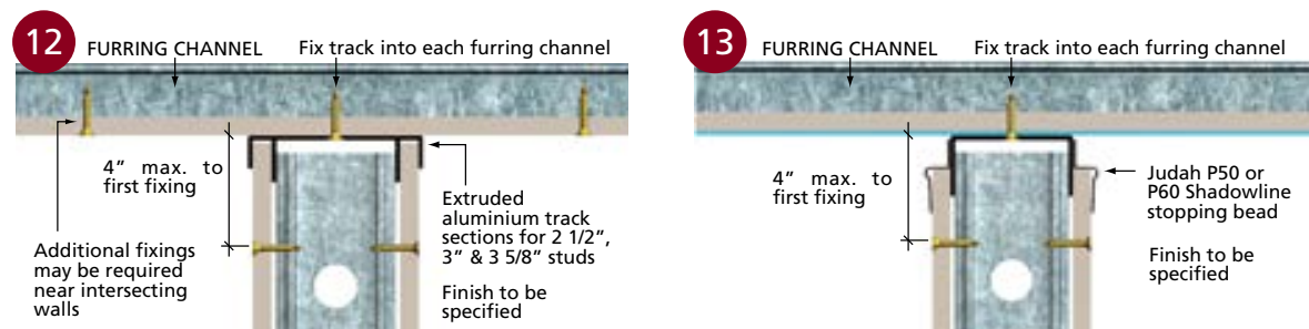
■ KEY-LOCK® CEILING
