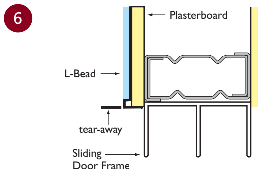
■ PTLB DETAIL
