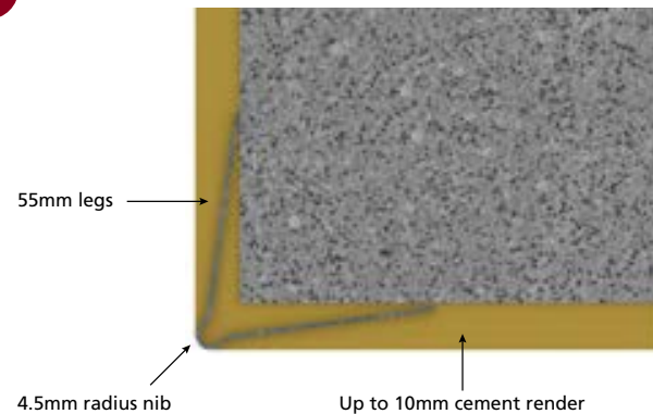
■ R01 CORNER BEAD DETAIL
