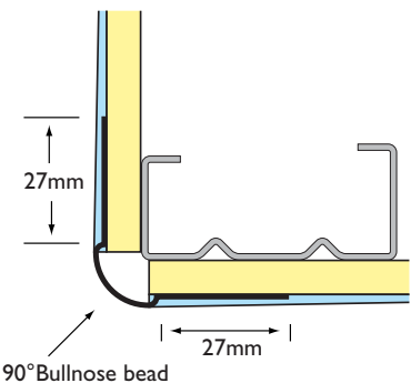
PBNA90 DETAIL
