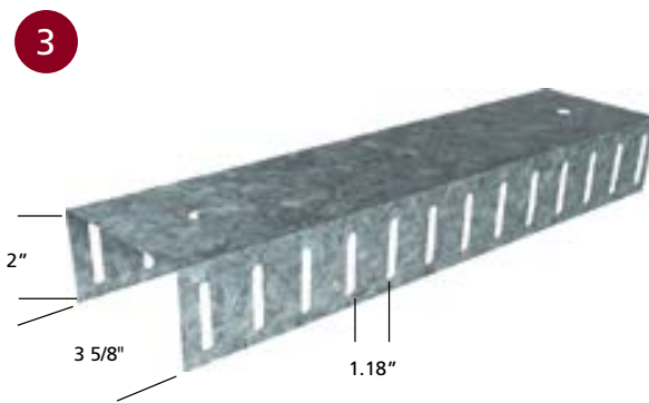
■ S683 MAXITRACK SLOTTED DEFLECTION HEAD TRACK
