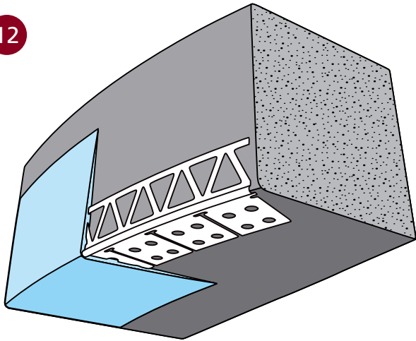
■ REA2530 DETAIL
