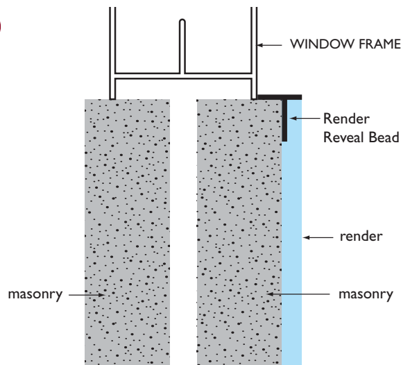
■ REVEAL BEAD DETAIL
