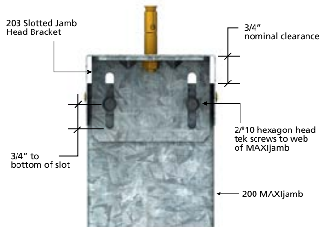
■ FIXING DETAILS FOR MAXIJAMB HEAD
