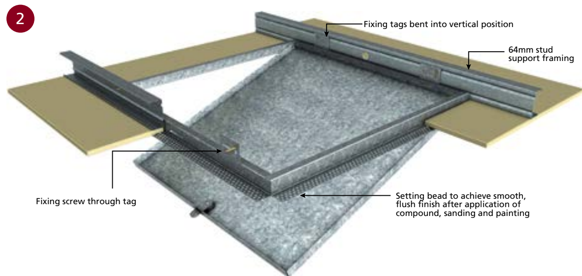
■ MFAP INSTALLATION
