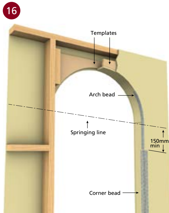
■ ARCH BEAD INSTALLATION
