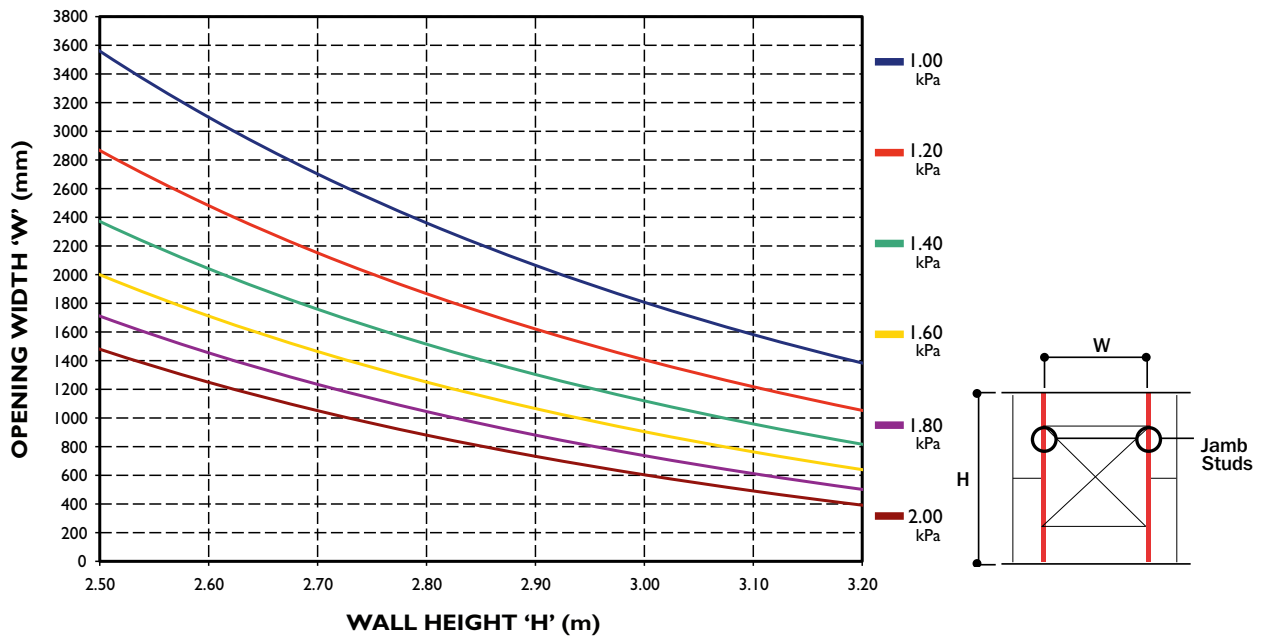
CHART J2: DESIGN REGION A — H/360
