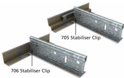
■ FIGURE 3: STABILISER CLIPS
