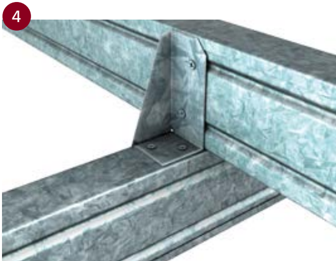
■ INSTALLATION OF THE SECONDARY PRIMARY SYSTEM
