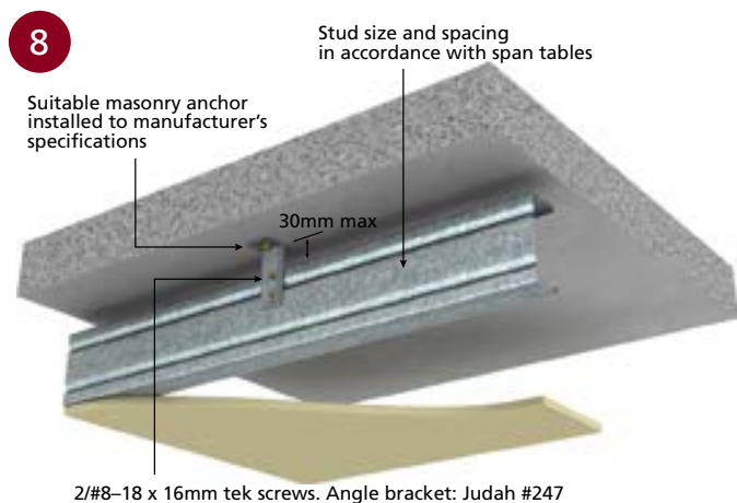
■ SUSPENSION JOINT TYPE 3
