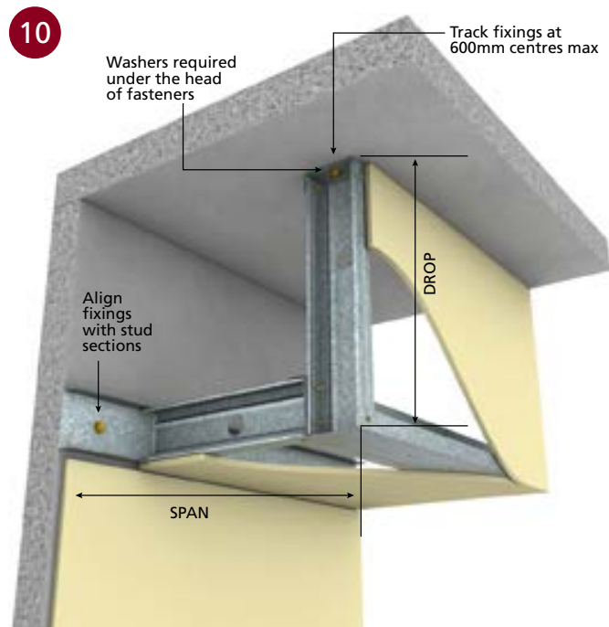
■ BOX-TYPE BULKHEAD
